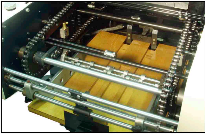
CHAIN DELIVERY with SPRAY UNIT and SELF OILING CHAINS
